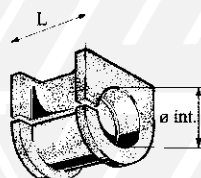
17 - 730338 \varnothing 24x55 18 - 730341 \varnothing 26x60 19 - 730337 \varnothing 28x60 20 - 730339 \varnothing 28x70 21 - 730342 \varnothing 32x70 22 - 730340 \varnothing 34x70
