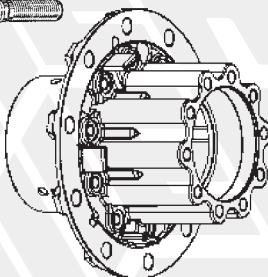
8 - 713949 nudo / bare NEW 9 - 713993 c/cuscinetti / c/w bearings
